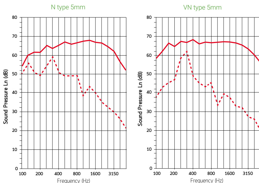
GRAPHS SHOWING REDUCTION OF IMPACT SOUND
