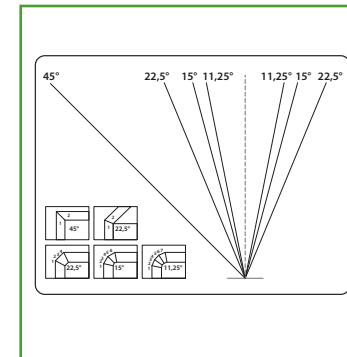
TEMPLATE (PRINTED ON TROCELLEN SLEEVE BOXES)
